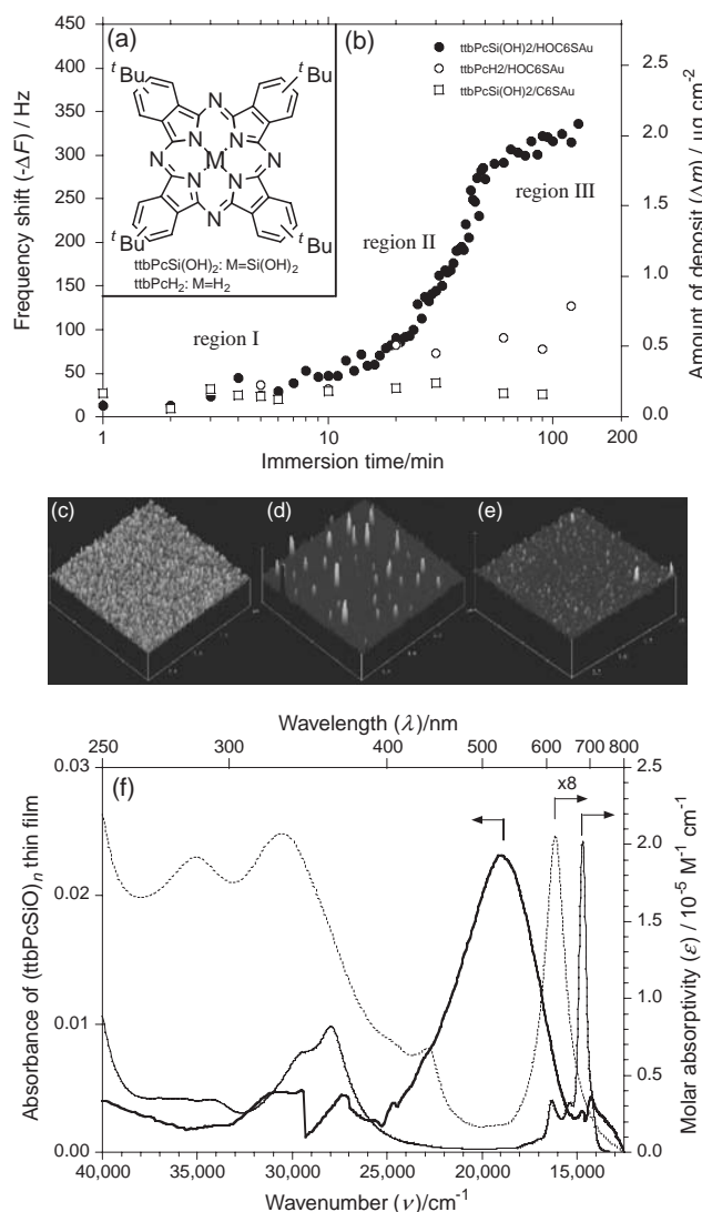
Figure 1. (a) Chemical structure of ttbPc derivatives in this work. (b) The amount of immobilized ttbPcSi(OH) 2 and ttbPcH 2 on the OH-coated gold surface, and ttbPcSi(OH) 2 on the alkane-coated gold surface by QCM method under 1.5 \times 10^{-5} M chloroform solution. Typical AFM images of the deposited thin film. [(c) 1 min, (d) 10 min, (e) 120 min; Area: 2 \times 2 μm, Height: 10 nm] (f) UV-vis spectra of the deposited thin film (thick solid line), ttbPcSi(OH) 2 (thin solid line), and oligo-(ttbPcSiO) n (thin dotted line) in CHCl 3 .
